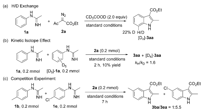
Scheme 5. Mechanistic studies.
